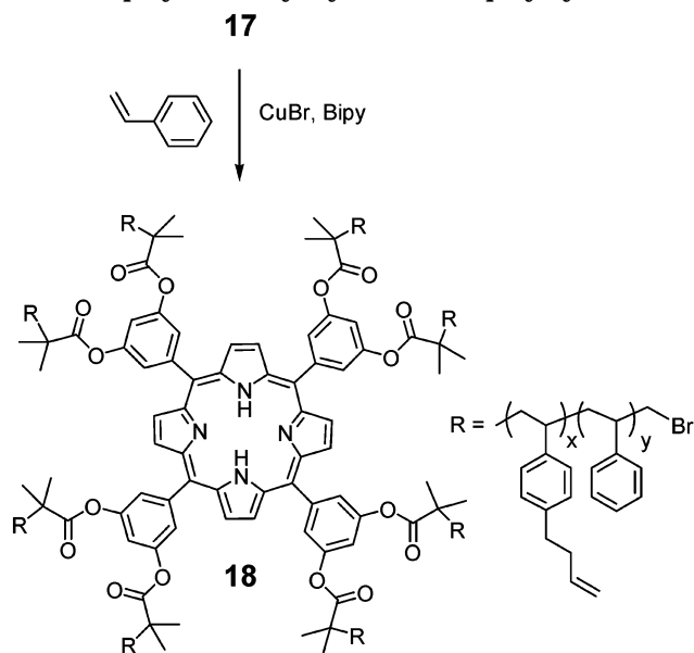
Scheme 9. Synthesis of Eight-Armed Star 18 , Star(poly-4-butenylstyrene- block -polystyrene)
